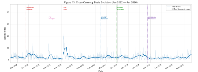
Figure 13: Full-history daily absolute basis (Jan 2022 to Jan 2026). Post-GENIUS Act basis compresses below historical baseline.
