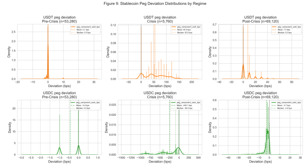
Figure 9: Stablecoin deviation distributions across regimes. USDT (top): safe-haven premium. USDC (bottom): massive de-peg during crisis.
