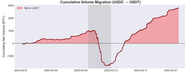
Figure 11: Cumulative volume migration (USDC → USDT). The sharp dip reflects USDC panic selling; the sustained climb to +3,000 BTC confirms permanent migration.
